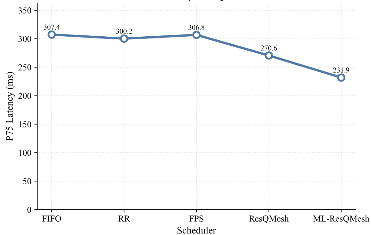
P75 Latency - Large Load
